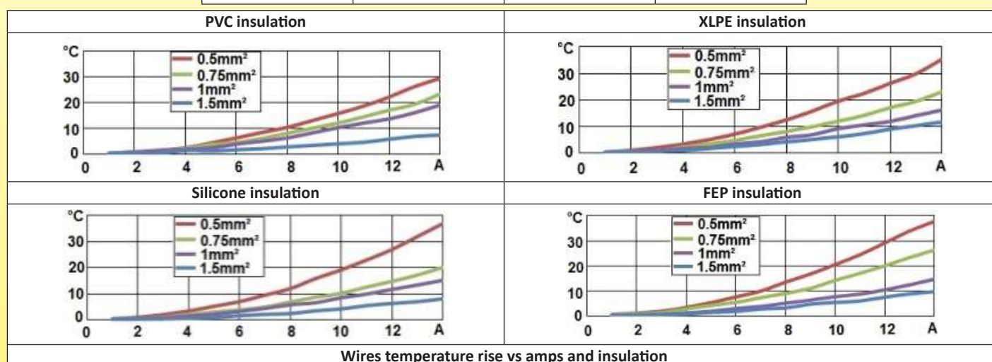
Wires temperature rise vs amps and insulation
